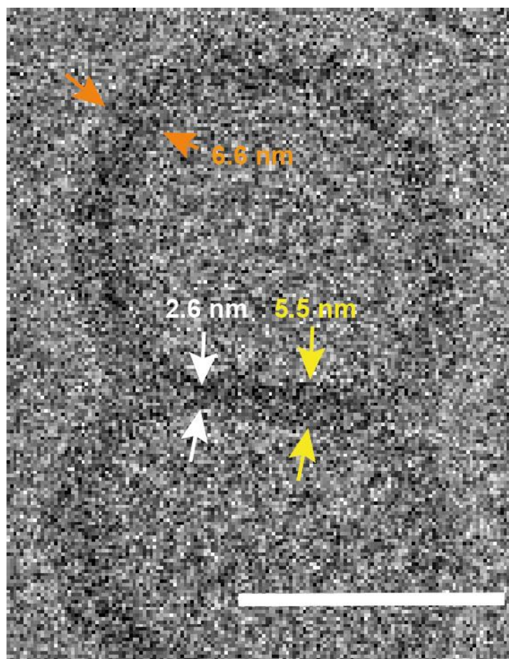
Fig. S13. Diaphragm thinning in fusing polymersomes. Membrane thinning (shown with white arrows) can be observed at the juncture, indicating the plausible location of eventual pore opening. For a comparison, the average diaphragm thickness (yellow) and the average polymer membrane thickness (orange) are also indicated. Scale bar = 30 nm.
