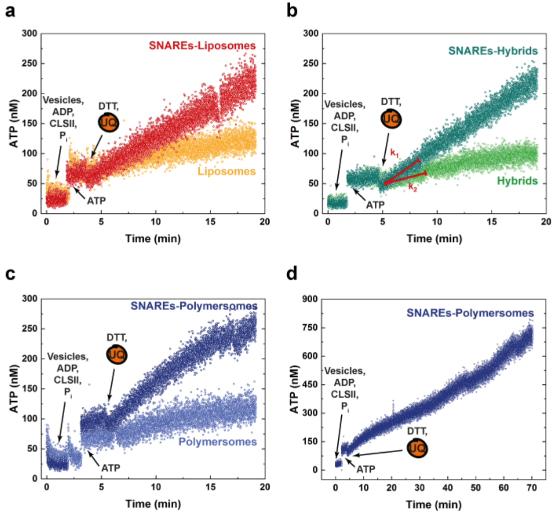
Fig. S10. SNARE-mediated content mixing of lipid, hybrid and polymer vesicles. Comparison between SNARE-induced and SNARE-free content mixing in lipid (a), hybrid (b) and polymer (c) vesicles detected via ATP synthesis. One population of vesicles, containing \Delta N complex and ATP synthase, was mixed with a second population, which contained synaptobrevin and bo_3 quinol oxidase in the presence of cofactors required for ATP synthesis and a luminescence assay (CLSII). After signal calibration with a known amount of ATP, ubiquinone along with the electron donor DTT were added to initiate proton pumping by bo_3 oxidase. The established proton gradient was used to drive ATP synthesis by the ATP synthase only in the case where both enzymes were integrated in same vesicles (i. e., upon successful fusion). The ATP synthesis rate of SNARE-containing vesicles ( k_1 ) and SNARE-free vesicles ( k_2 ) were determined from the initial rates. While the comparatively lower ATP synthesis in SNARE-free vesicles was seen to subside after several minutes, high ATP synthesis rates were sustained in SNARE-containing vesicles over prolonged period of time. (d) Extended SNARE-induced content mixing in polymer vesicles.
